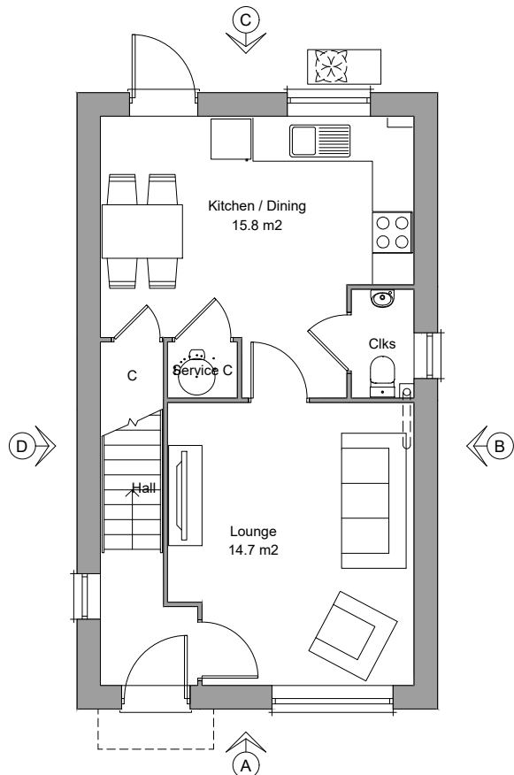
Ground Floor Plan Area 40.0m²
