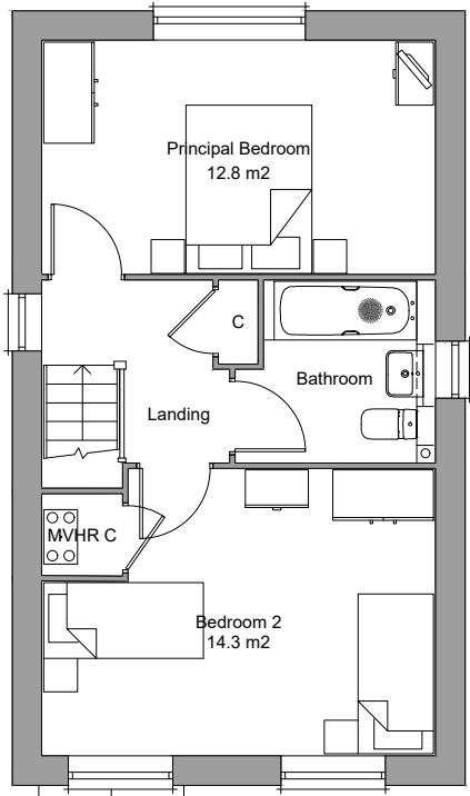
First Floor Plan Area 40.0m²
