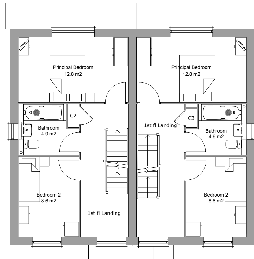
First Floor Plan Area 40.0m²
