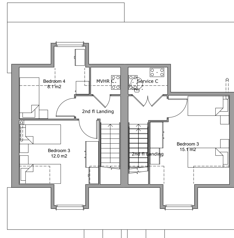
Second Floor Plan Area 28.3m²
