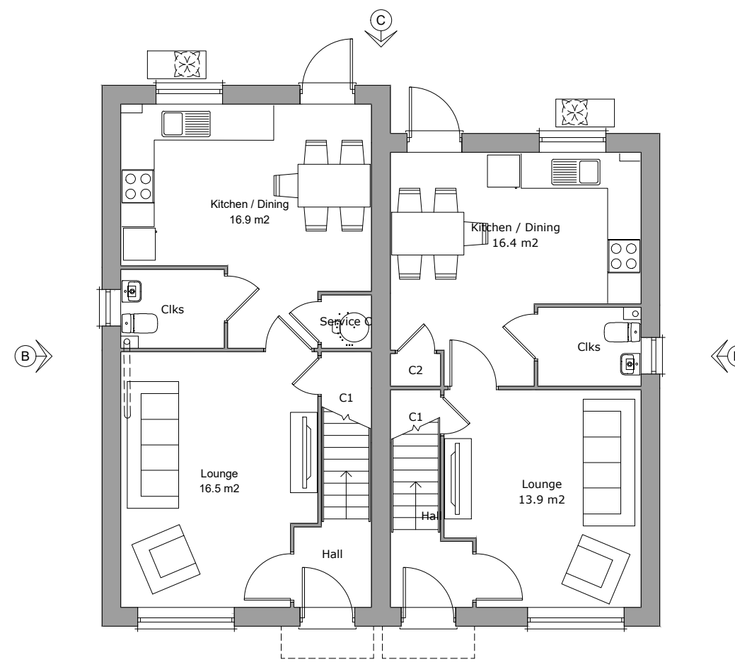
Ground Floor Plan Area 44.2m²
