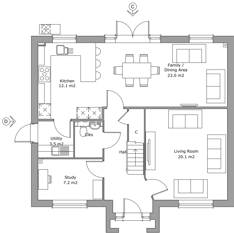
Ground Floor Plan Area 84.1m²
