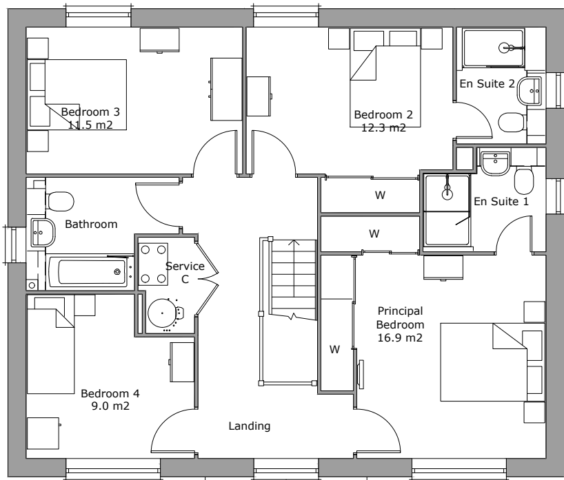
First Floor Plan Area 82.7m²
