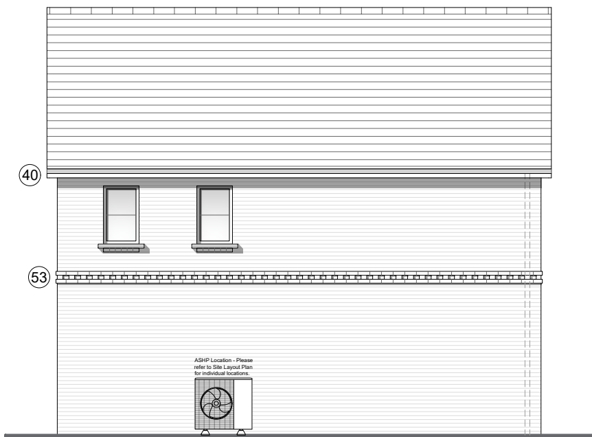
Elevation C Plots 87 Handed
