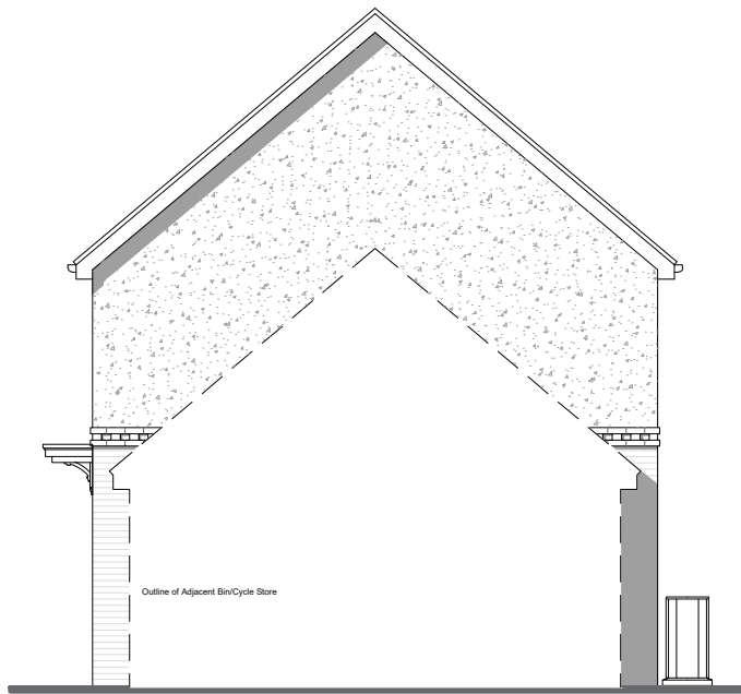
Elevation D Plots 115 As
