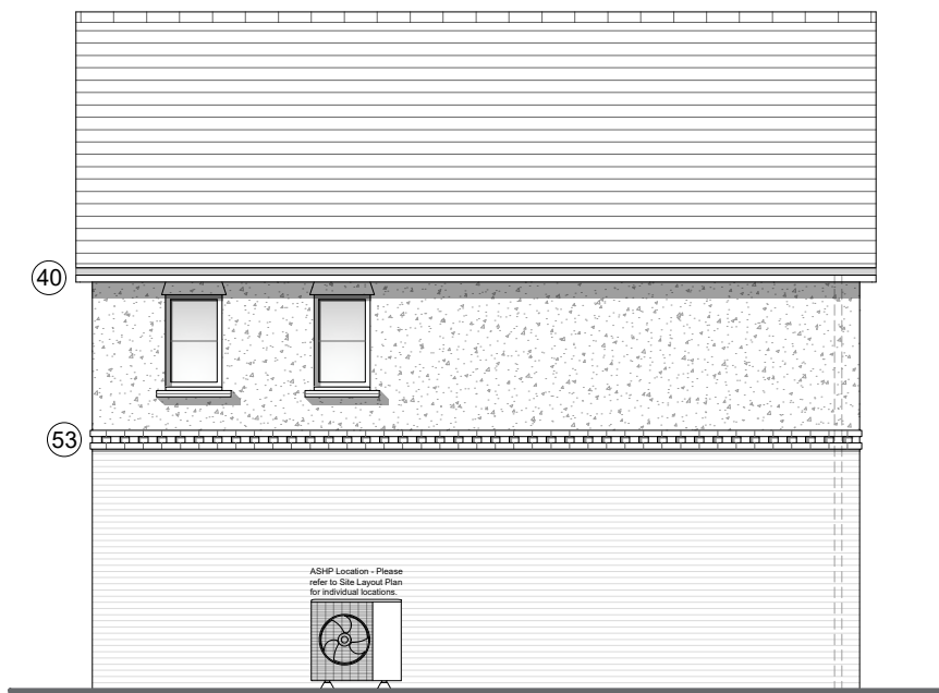
Elevation C Plots 115 As
