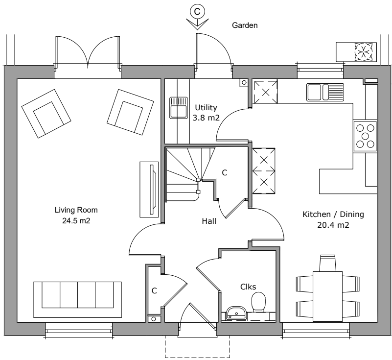
Ground Floor Plan Area 64.3m 2
