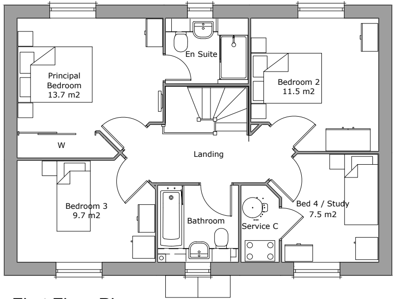
First Floor Plan Area 64.3m 2
