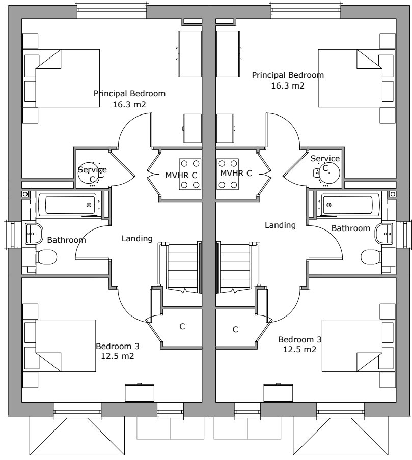
Second Floor Plan Area 46.8m 2
