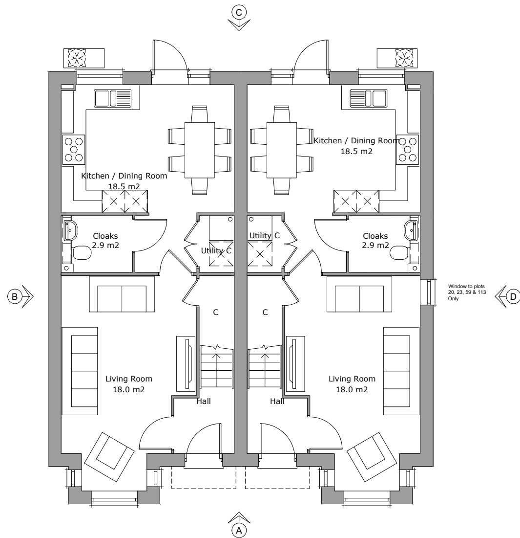
Ground Floor Plan Area 48.6m 2
