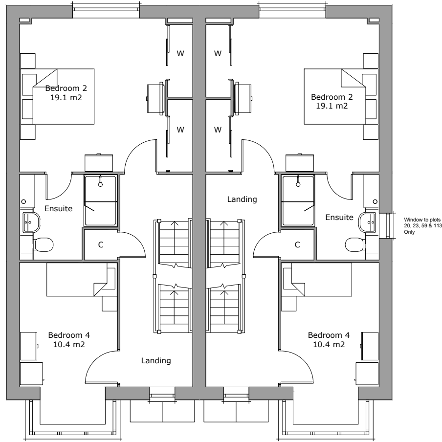
First Floor Plan Area 48.6m 2
