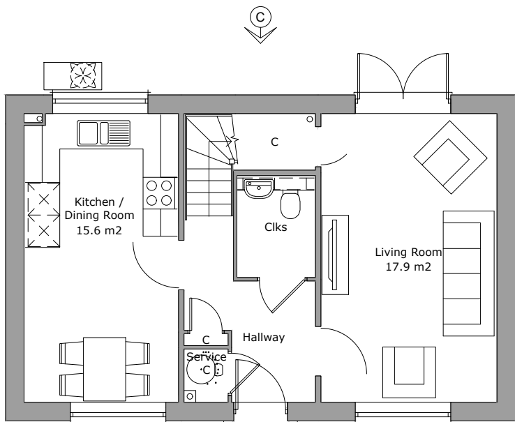
Ground Floor Plan Area 49.1m 2
