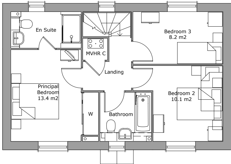
First Floor Plan Area 49.1m 2
