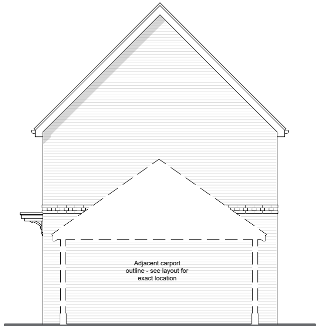
Elevation D
