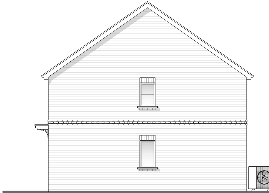
Elevation D
