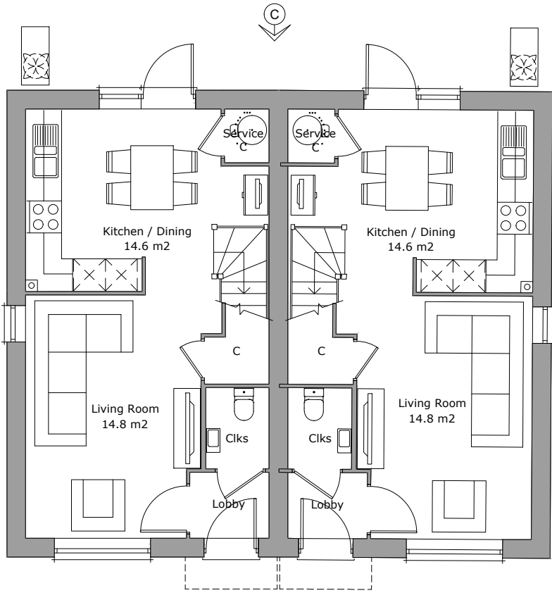
Ground Floor Plan Area 36.9m²
