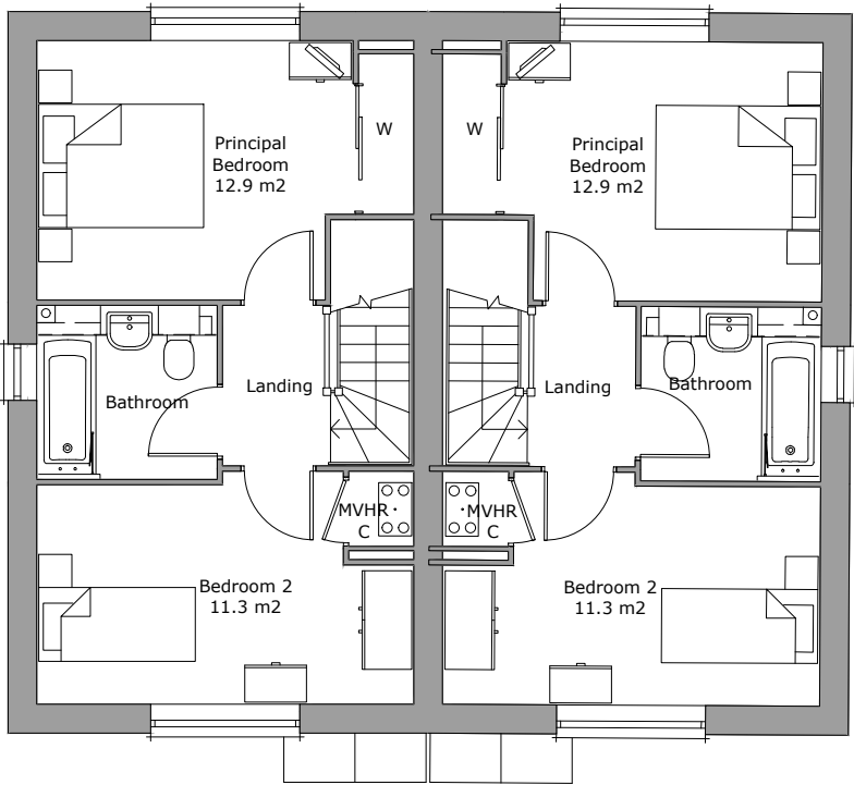
First Floor Plan Area 36.9m²
