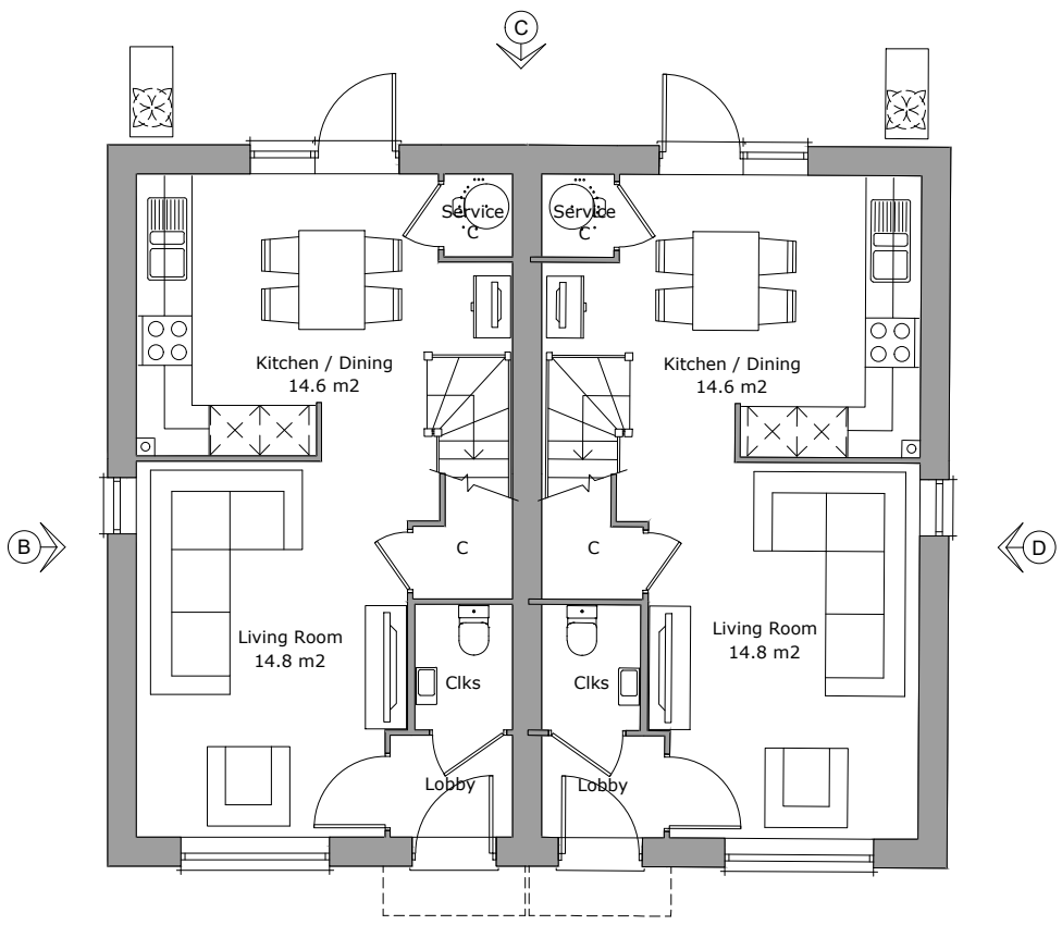
Ground Floor Plan Area 36.9m 2
