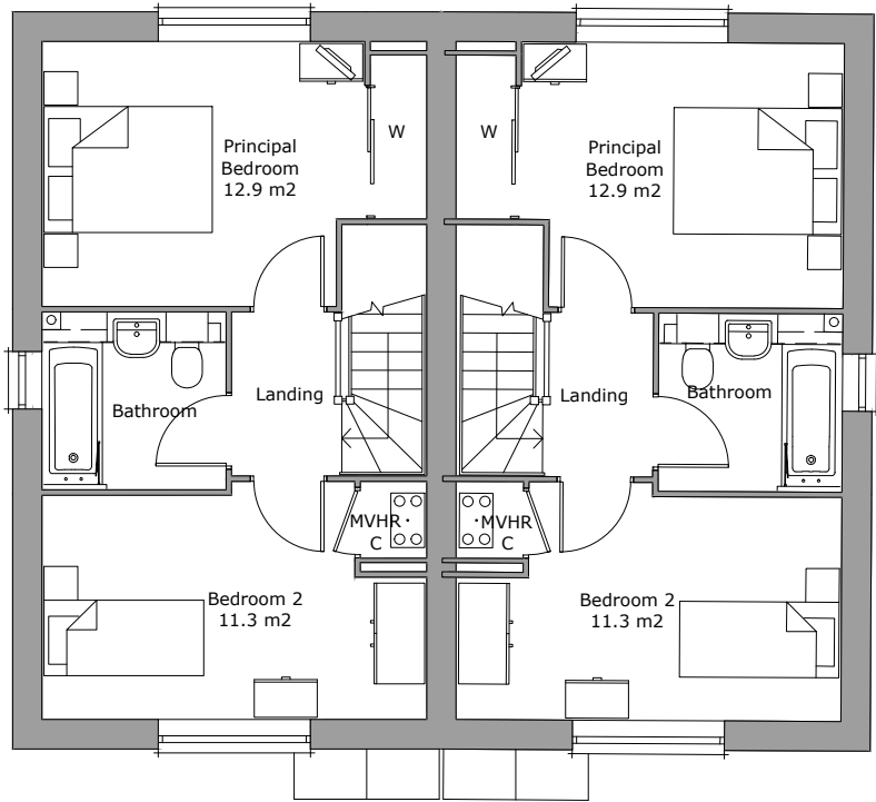
First Floor Plan Area 36.9m 2
