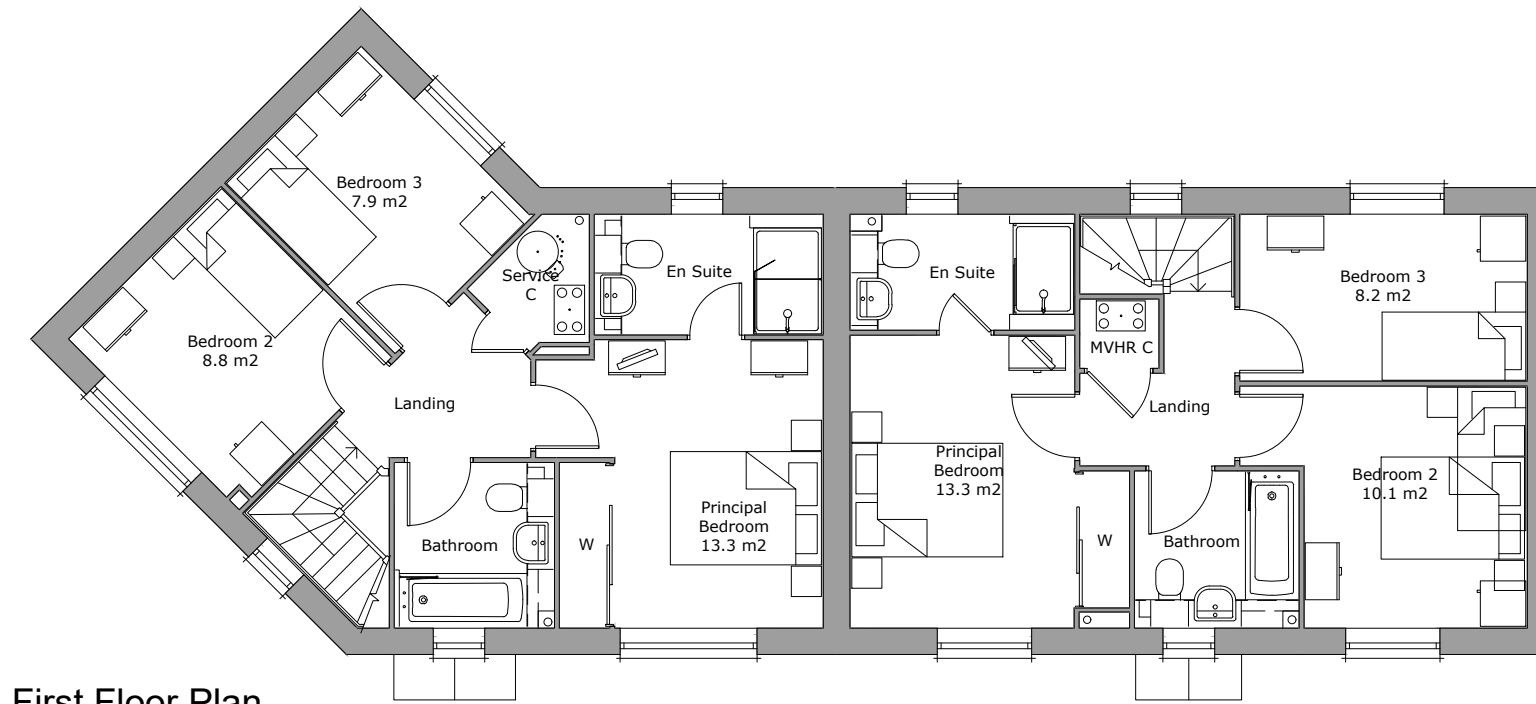
First Floor Plan Area 50.9m²
