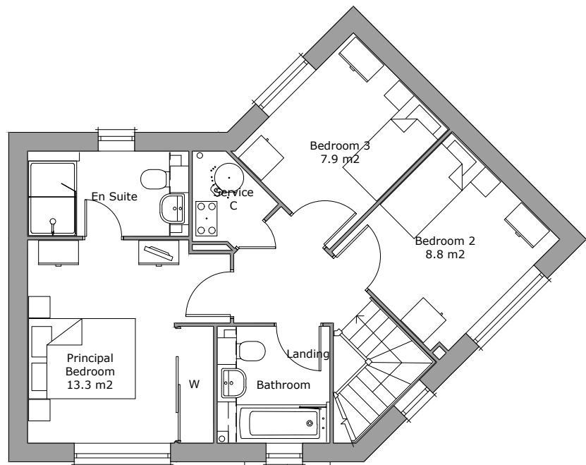
First Floor Plan Area 50.9m²
