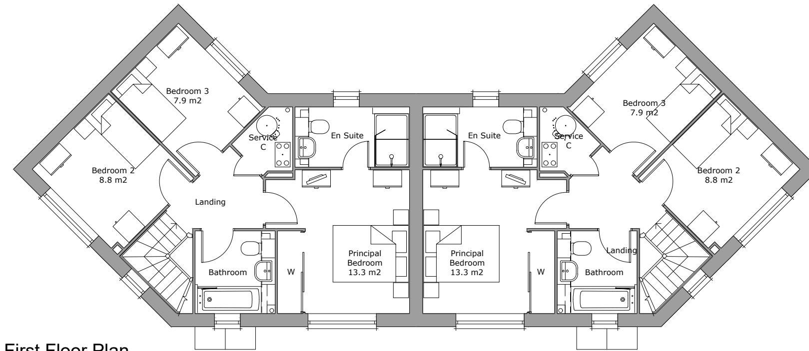
First Floor Plan Area 50.9m 2
