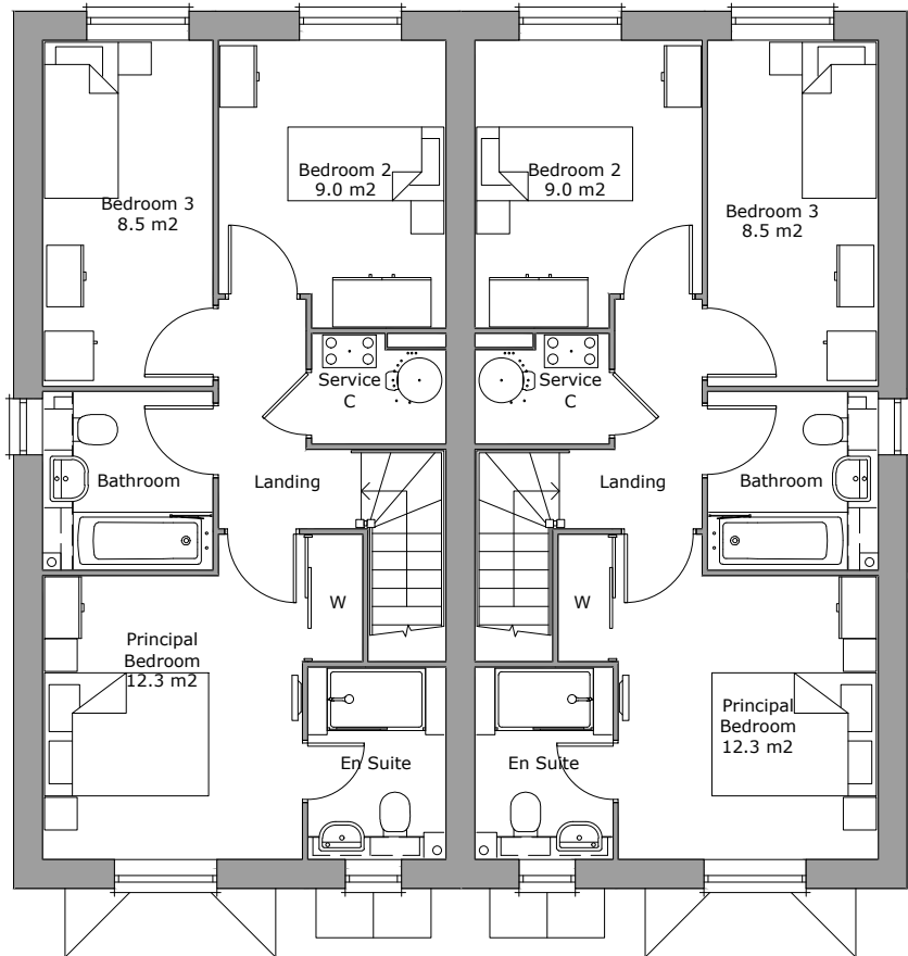
First Floor Plan Area 49.0m²
