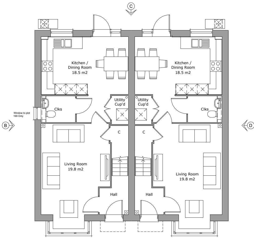
Ground Floor Plan Area 50.4m²
