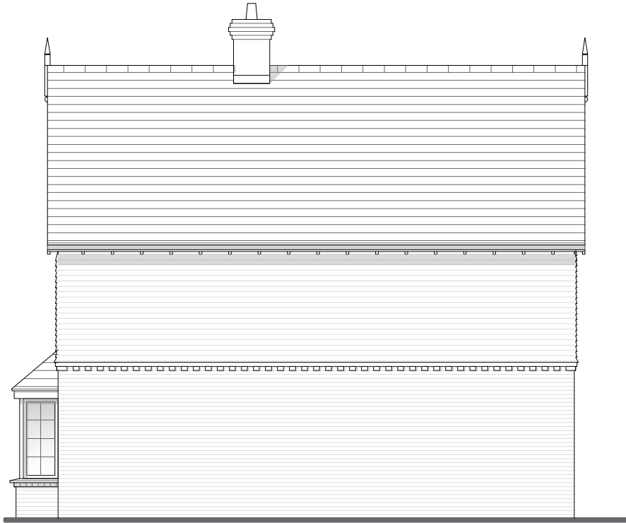
Elevation C
