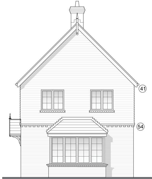
Elevation D
