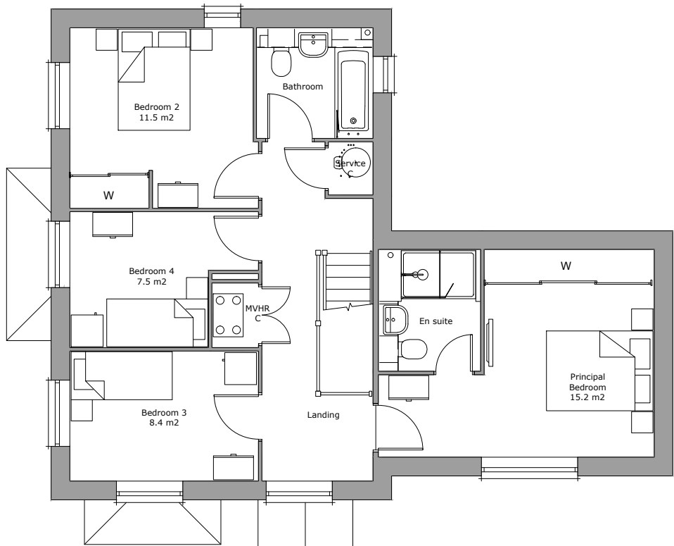
First Floor Plan Area 69.2m²
