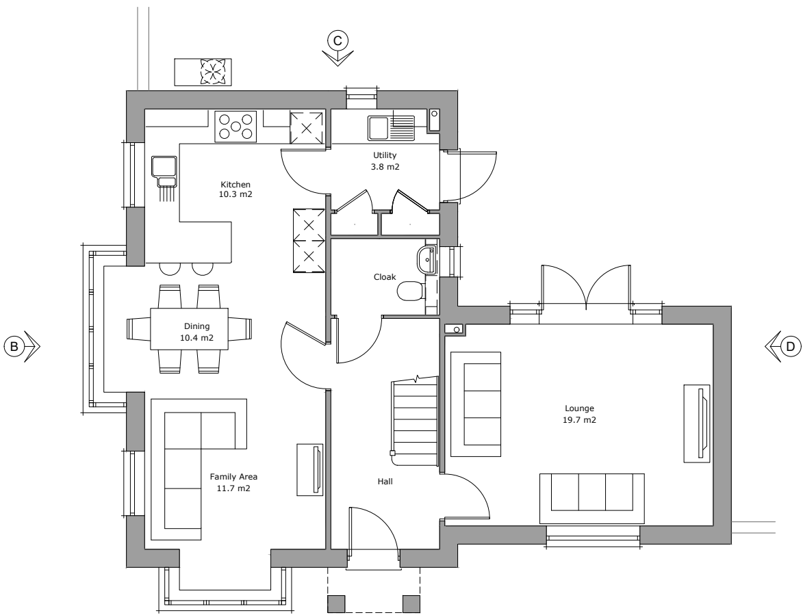
Ground Floor Plan Area 72.5m²
