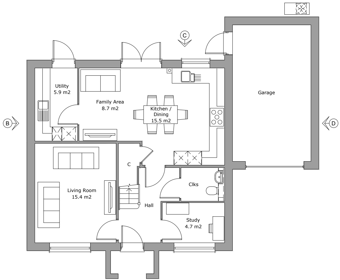
Ground Floor Plan Area 64.9m²
