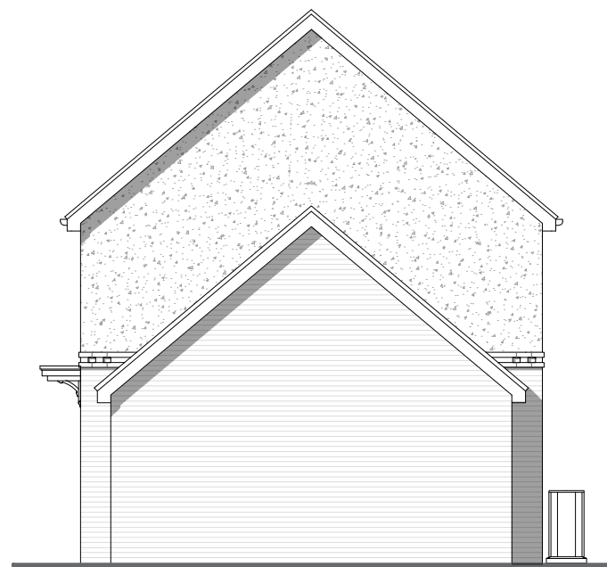
Elevation D Plots 86 As
