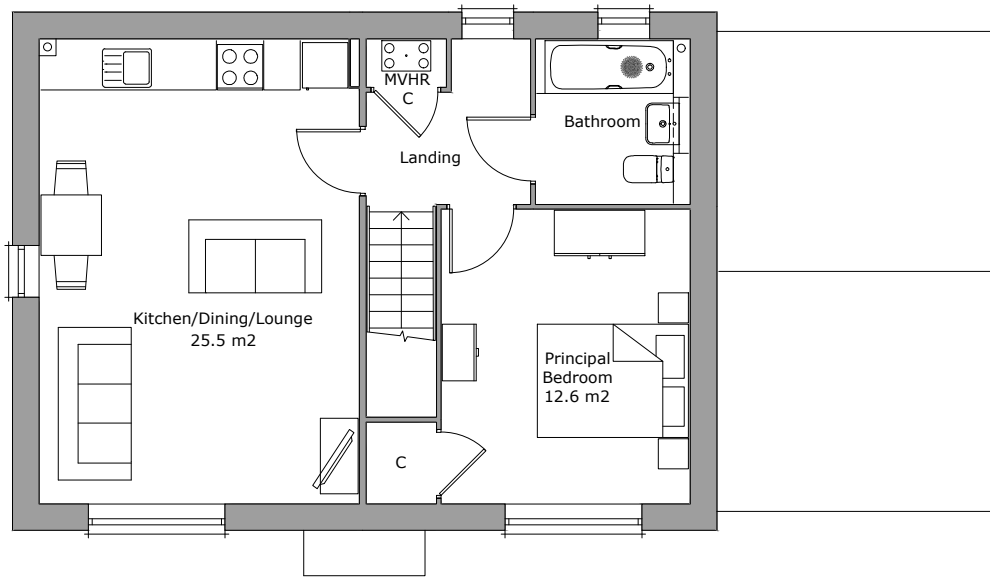
First Floor Plan Area 53.0m²
