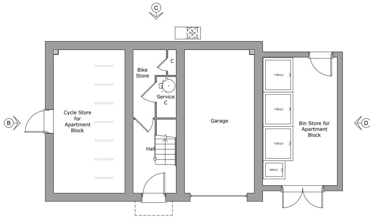
Ground Floor Plan Area 11.4m²
