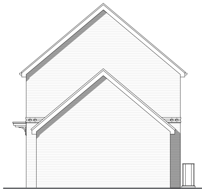
Elevation D Plots 116 Handed
