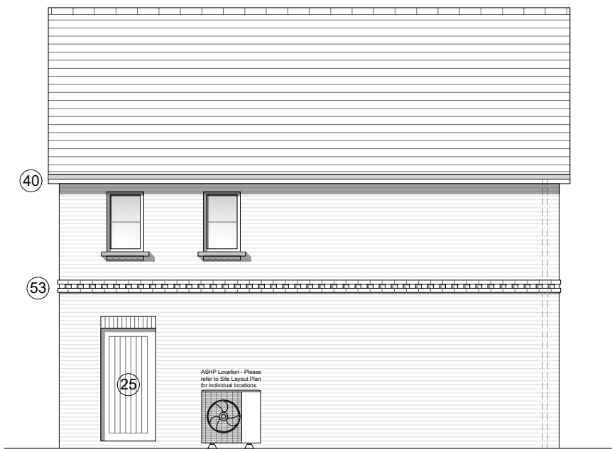
Elevation C Plots 108 Handed
