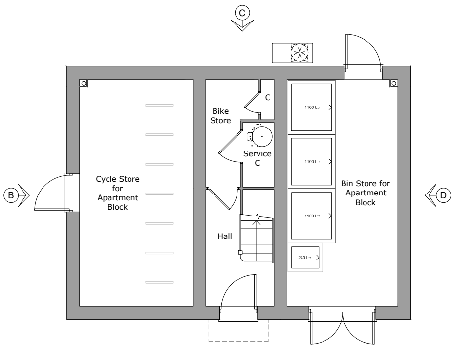
Ground Floor Plan Area 11.4m²
