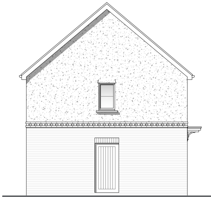
Elevation B Plots 143 As
