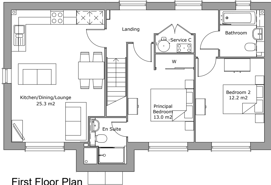
First Floor Plan Area 74.5m²
