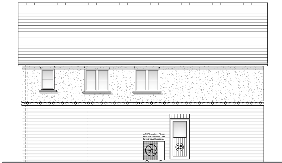
Elevation C
