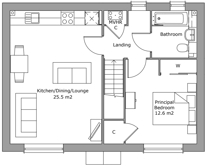
First Floor Plan Area 53.0m²
