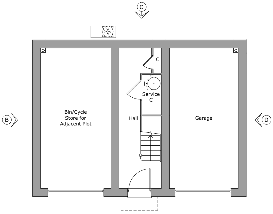
Ground Floor Plan Area 11.4m²
