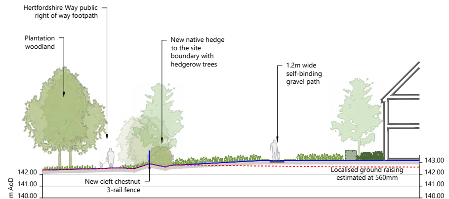
Section E - Proposed North Western Boundary
