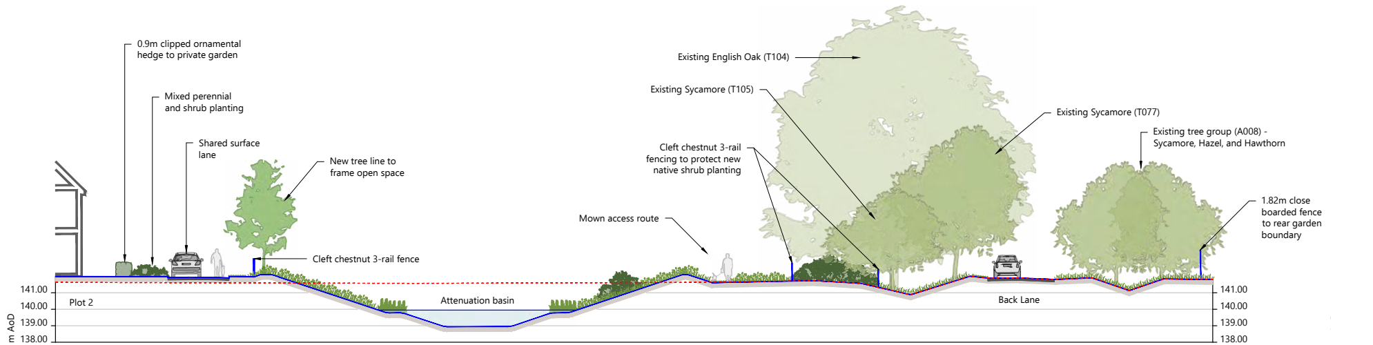
Section A - Proposed Southern Boundary
