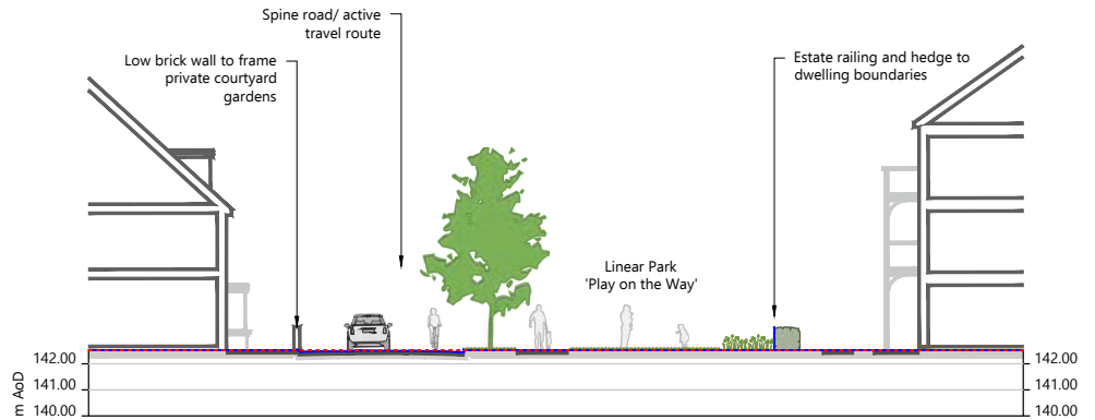
Section I - Proposed Linear Park
