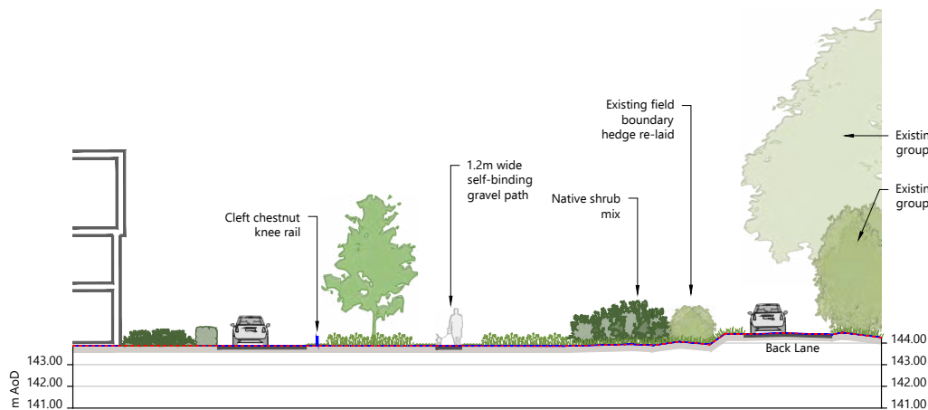
Section D - Proposed Eastern Boundary
