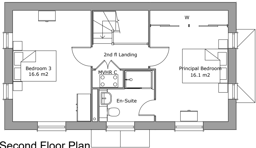
Second Floor Plan Area 46.8m²
