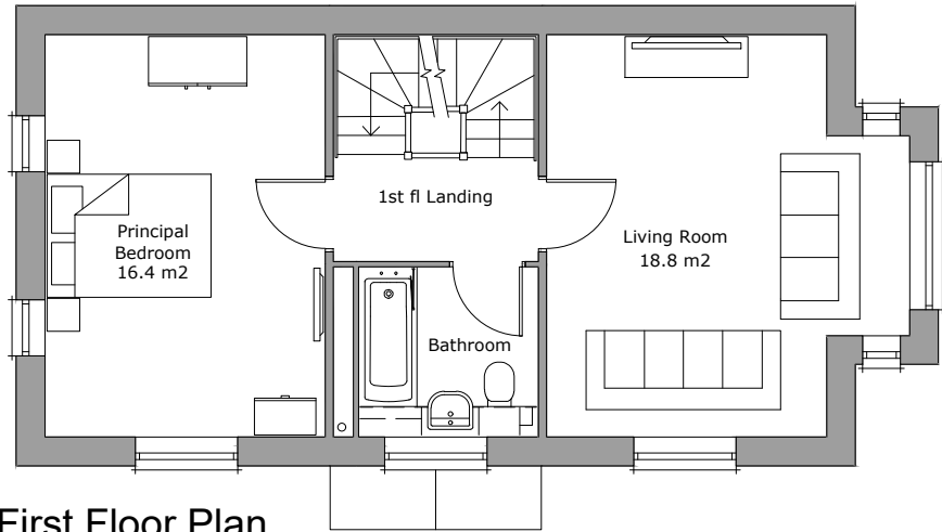
First Floor Plan Area 49.3m²
