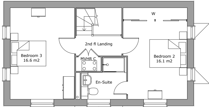
Second Floor Plan Area 46.8m²
