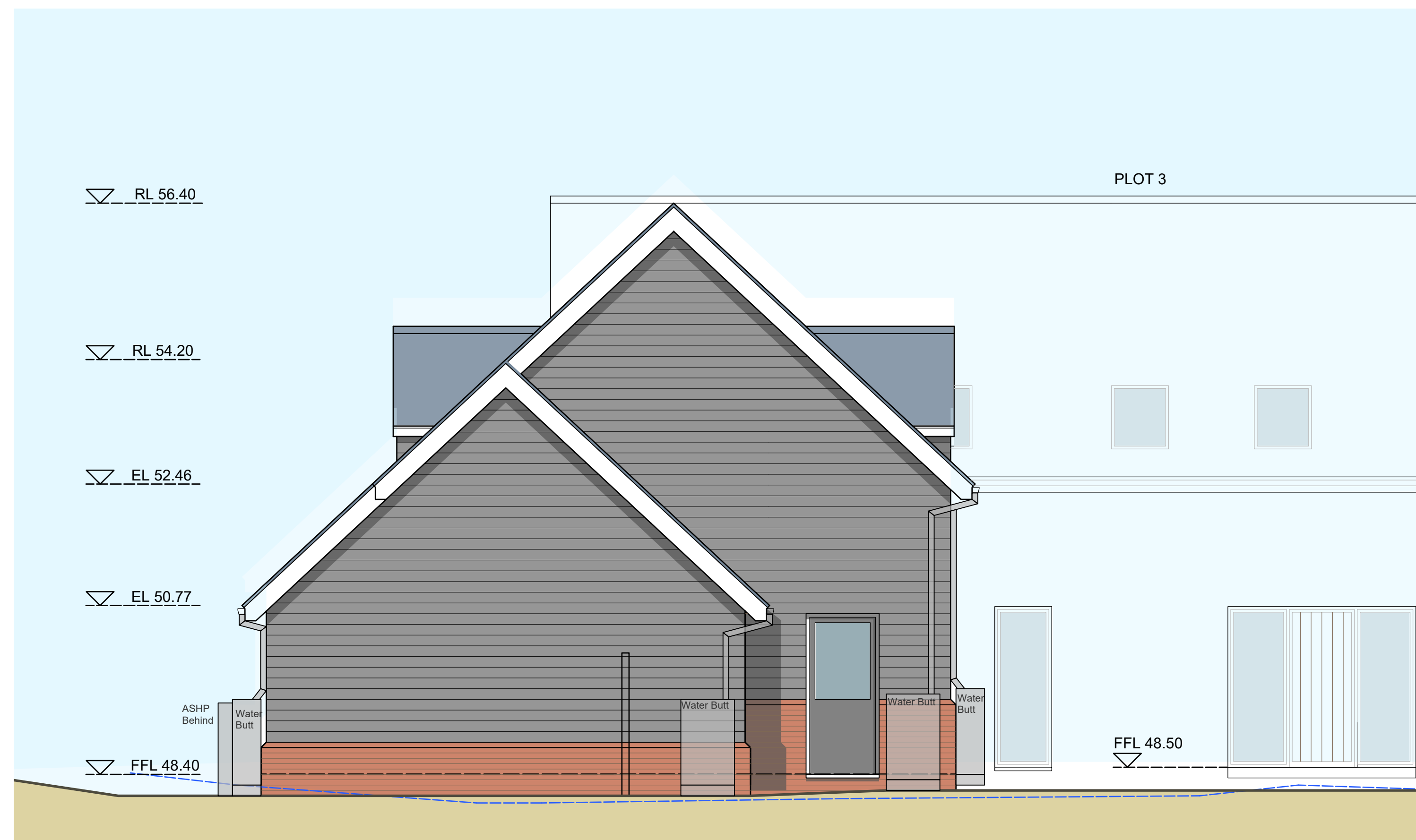
South Elevation
