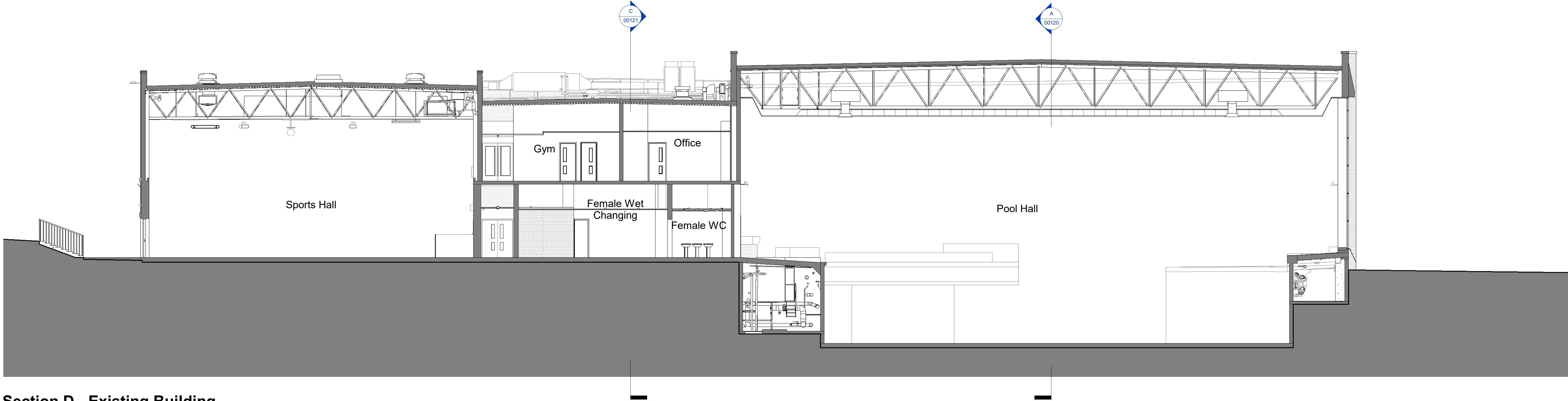
Section D - Existing Building 1 : 100
