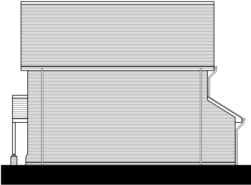
SIDE ELEVATION (C-C)
