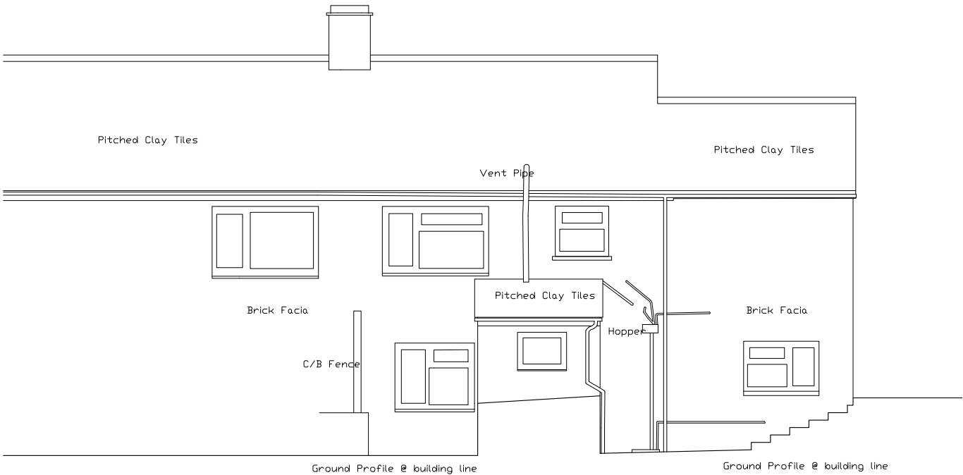
Elevation CC as Existing
