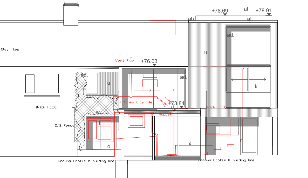
North elevation as Proposed
