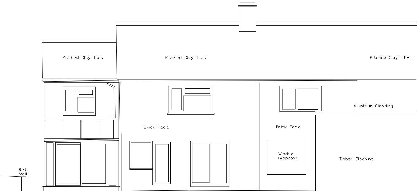
Elevation BB as Existing
