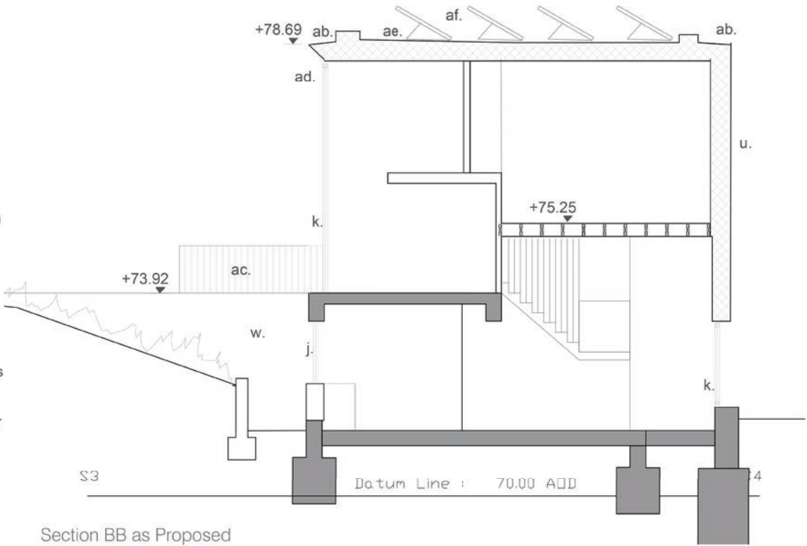
Section BB as Proposed
