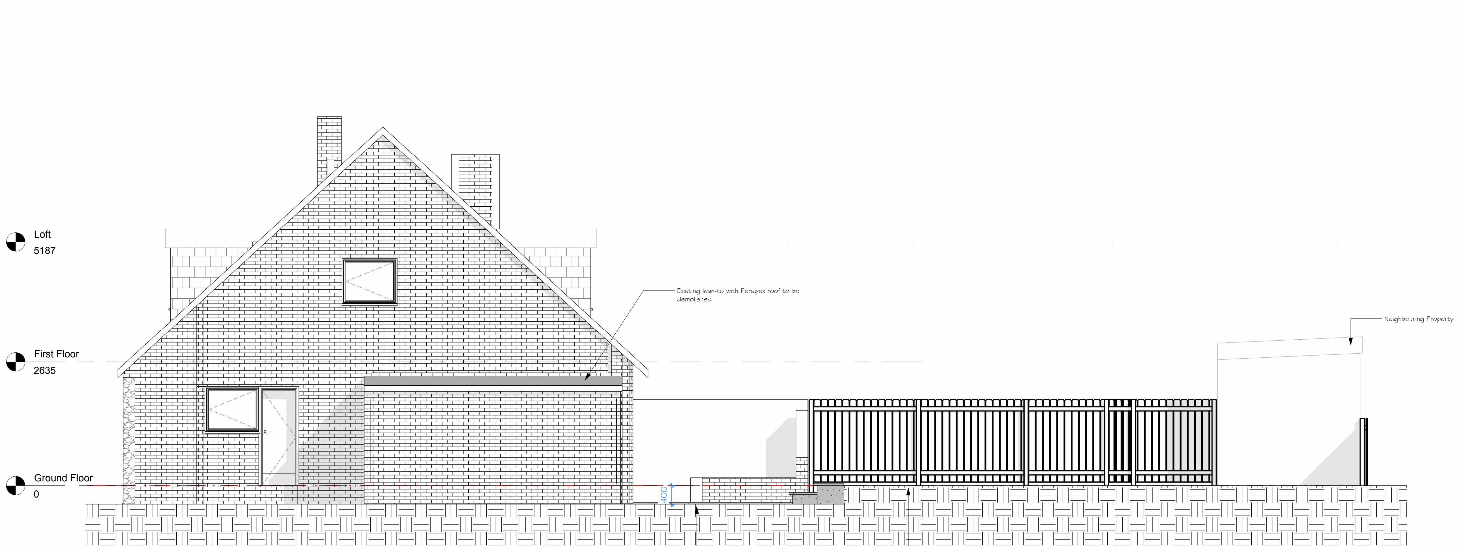
3 Existing External Elevation 1 : 50
