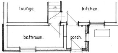
Proposed: Plan
