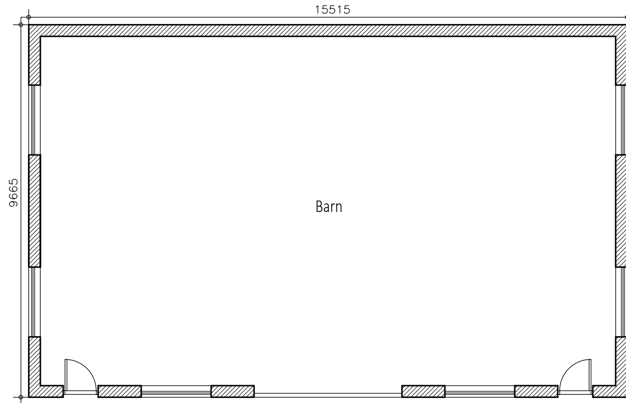
Floor Plan @ 1/100
