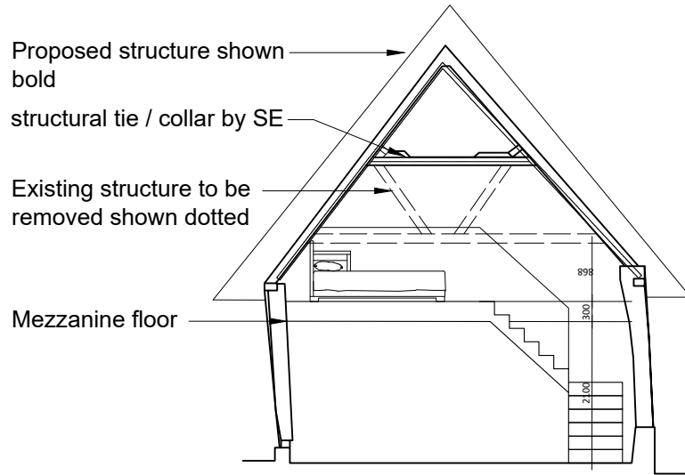
PROPOSED (approved) SECTION ELEVATION
