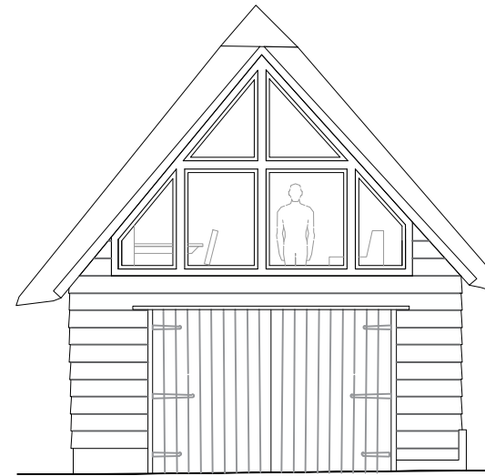
PROPOSED END ELEVATION
