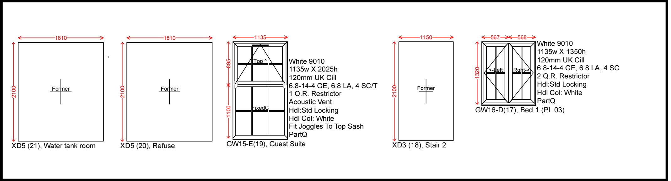
GROUND FLOOR - East Elevation (GF)
