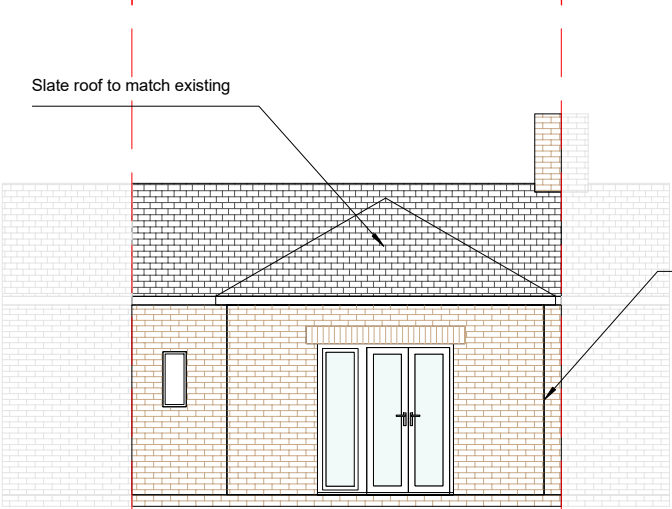
Proposed Rear (N) Elevation 1:100 Scale
