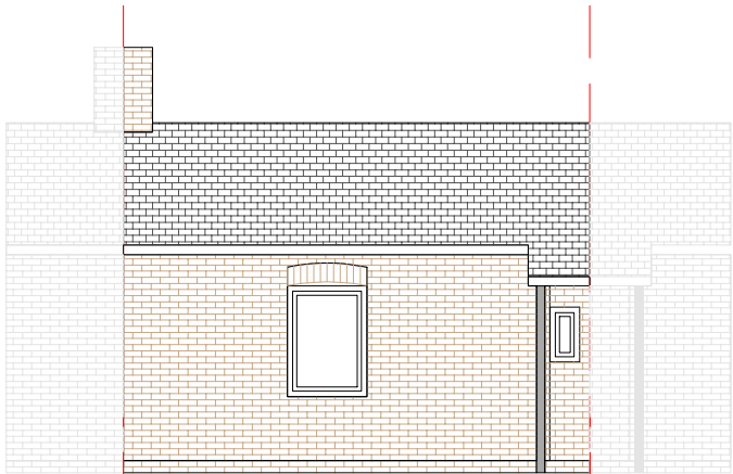
Existing Front (S) Elevation 1:100 Scale
