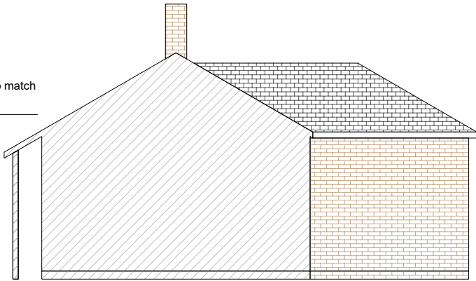
Proposed Side (E) Elevation 1:100 Scale
