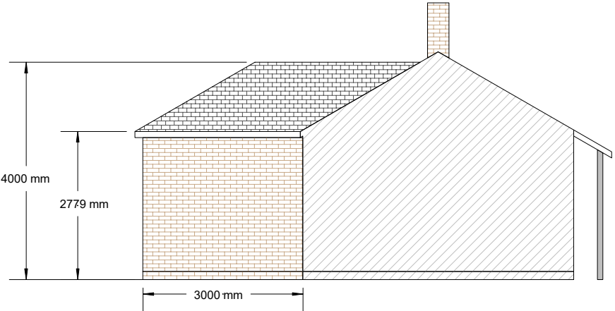
Proposed Side (W) Elevation 1:100 Scale
