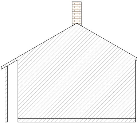
Existing Side (E) Elevation 1:100 Scale
