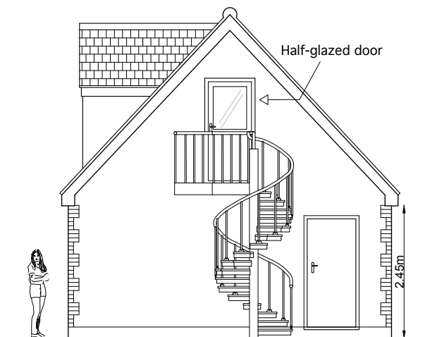
PROPOSED WEST FACING ELEVATION (FACING HOUSE)
