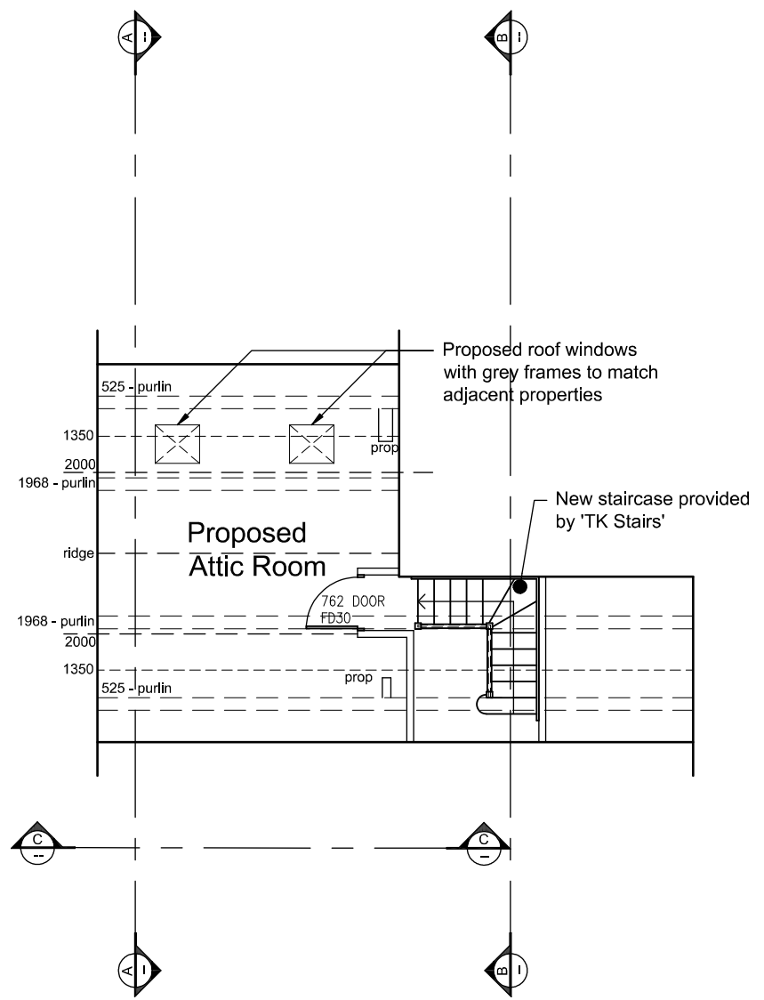
Attic Plan Scale - 1:100
