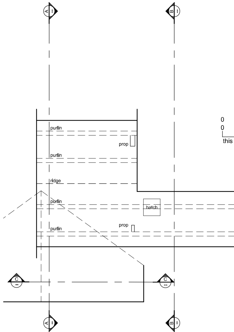
Attic Plan Scale - 1:100
