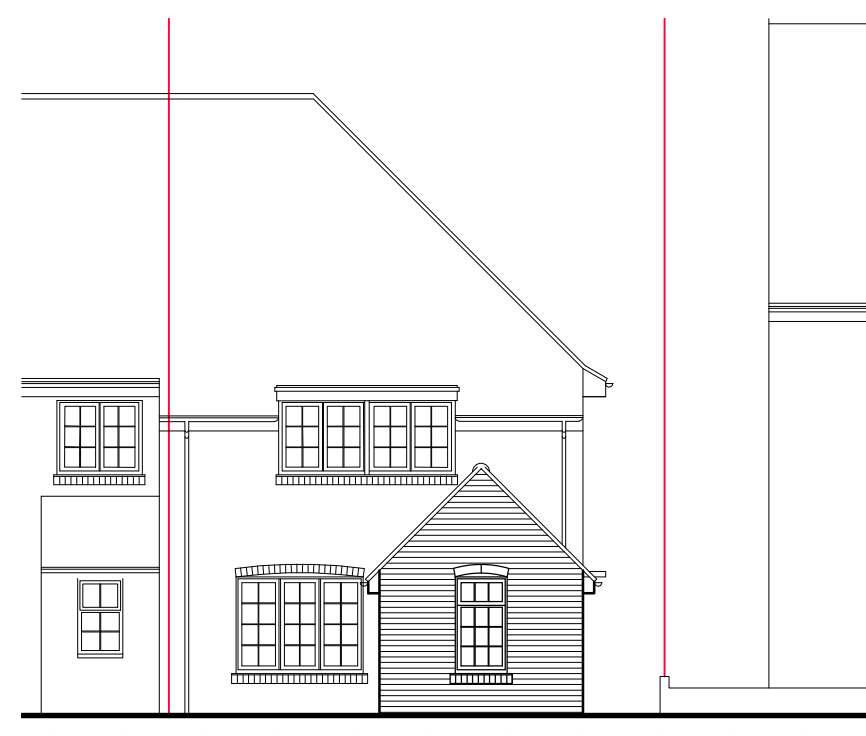
FRONT ELEVATION (VIEWED FROM PUBLIC FOOTPATH LEVEL) – PROPOSED (1:100)
