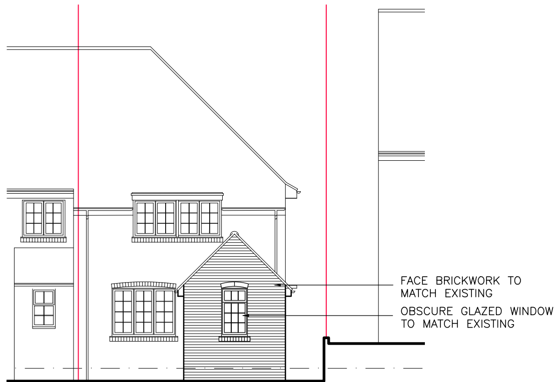
FRONT ELEVATION – PROPOSED (1:100)
