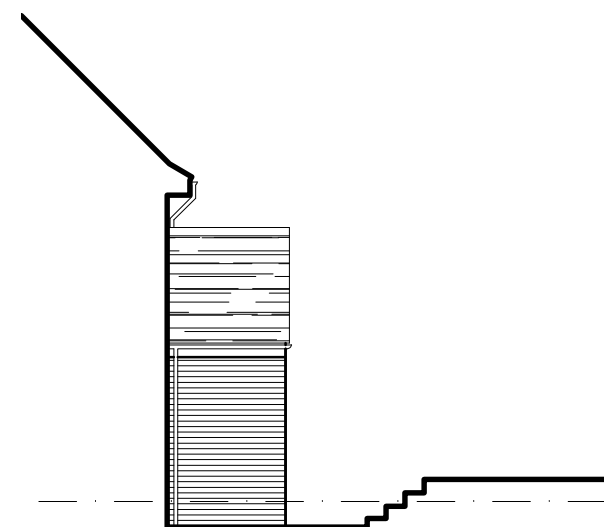
SIDE ELEVATION TO No. 92 – PROPOSED (1:100)
