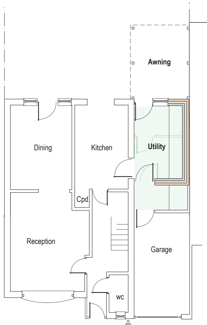
Ground Floor Plan (11m2)
