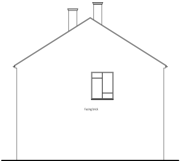
Side Elevation @ 1/100
