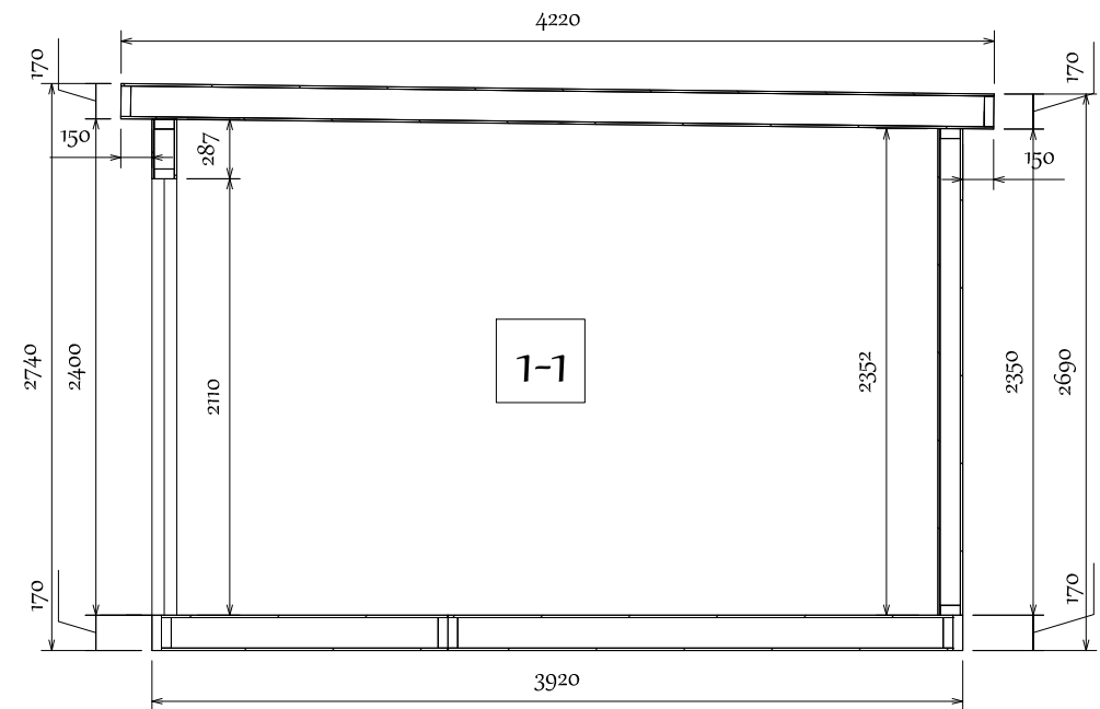
Sections
