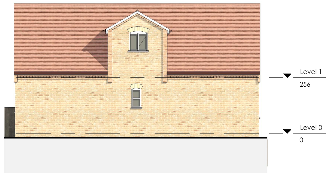
Proposed Left Elevation 1:100
