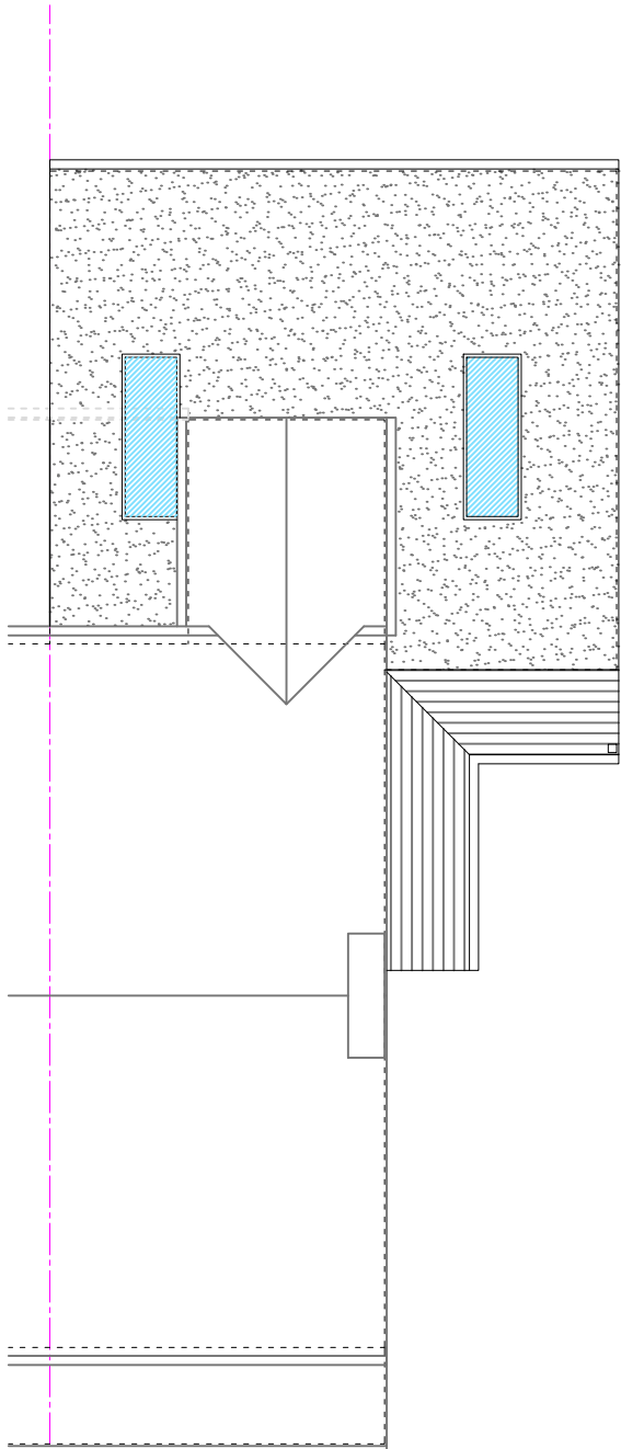
ROOF PLAN
