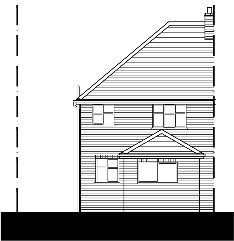
REAR ELEVATION (C-C)
