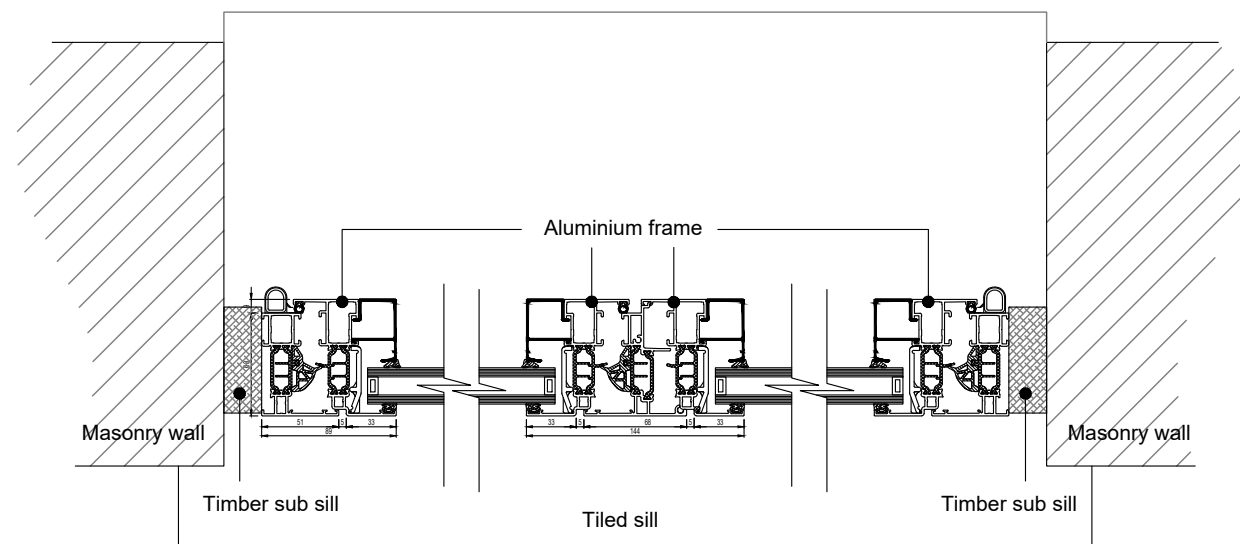
Plan detail of window 1:5
