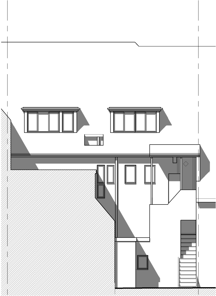
Existing North Elevation 1 : 100
