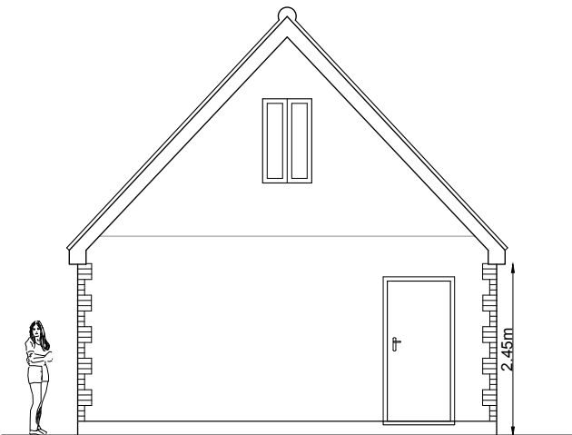
EXISTING WEST FACING ELEVATION (FACING HOUSE)
