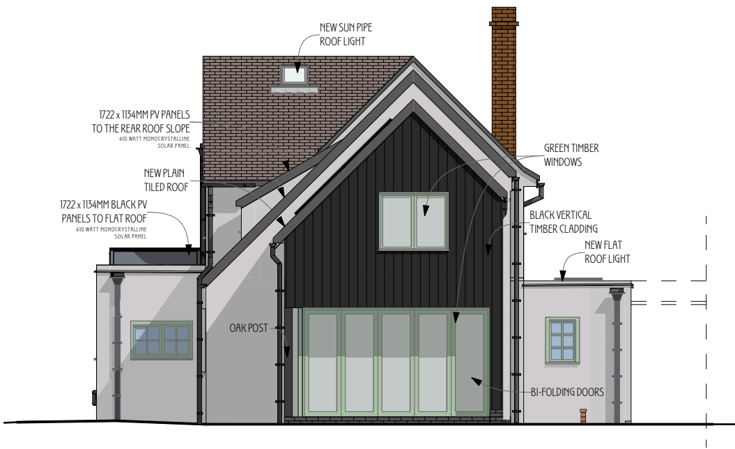
E-01 North-West Elevation 1:100
