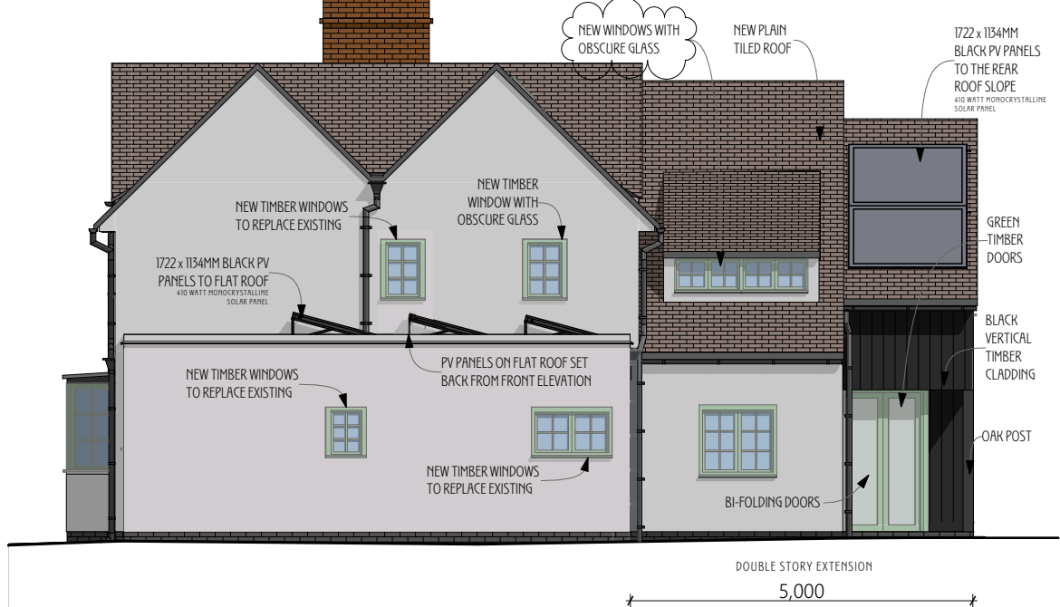
E-02 North-East Elevation 1:100
