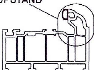
REBATE UPSTAND
