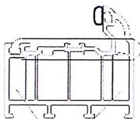
DRAINAGE CHAMBER
