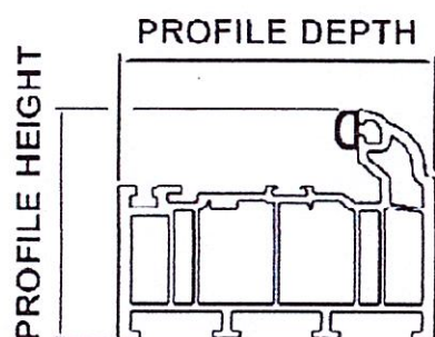
DRAINAGE PLATFORM
