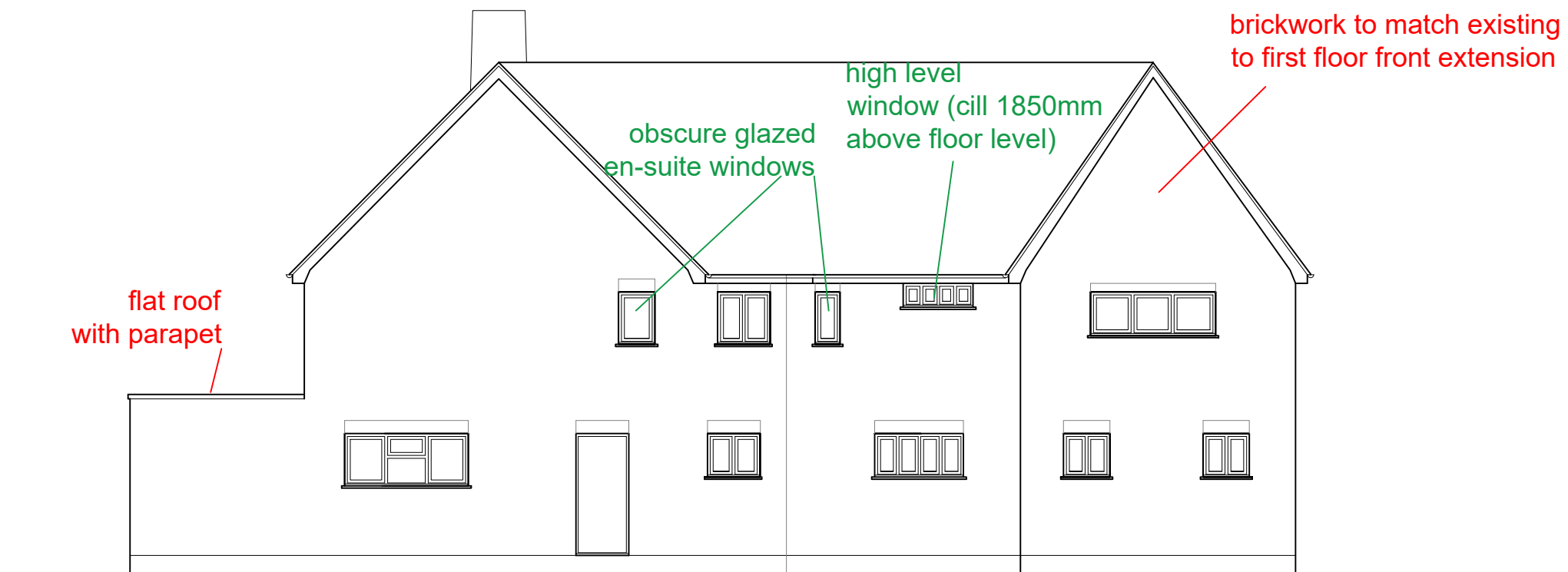
SIDE ELEVATION
