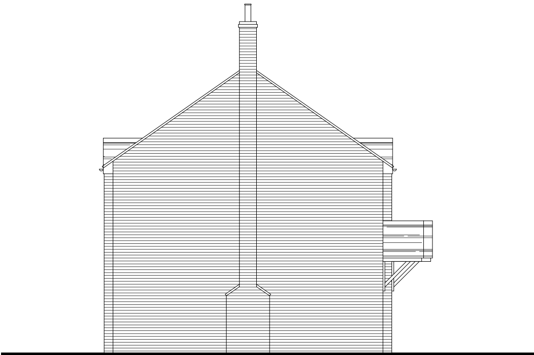
SIDE ELEVATION (1:100)
